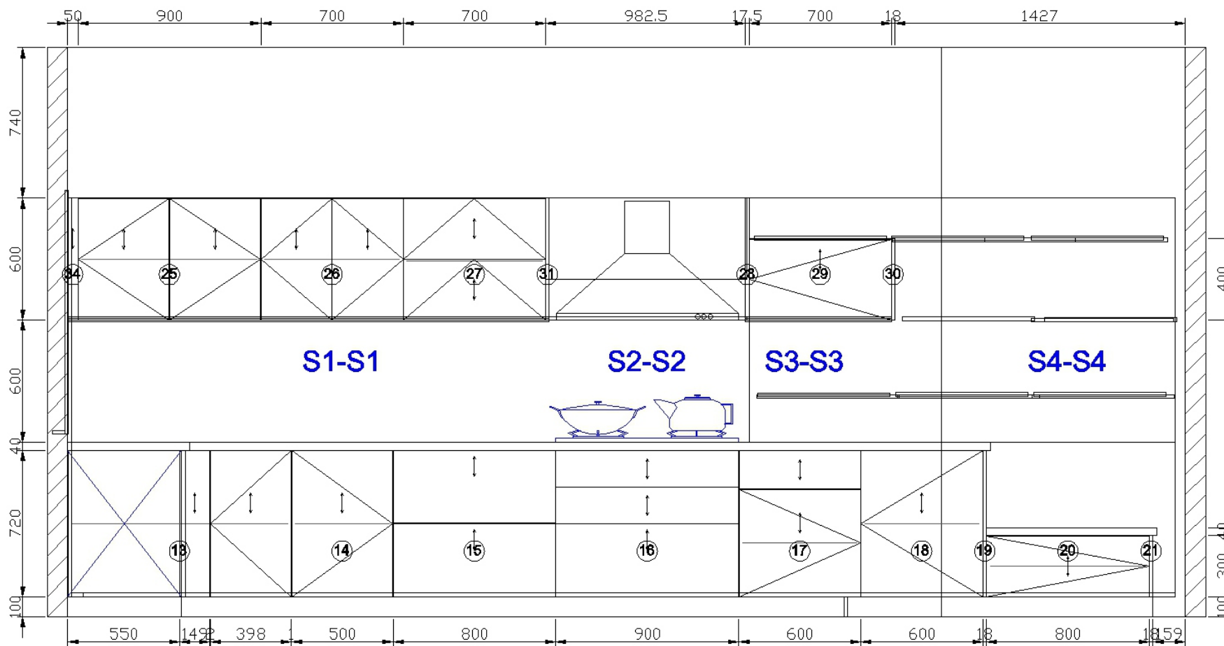
C View elevation drawing
