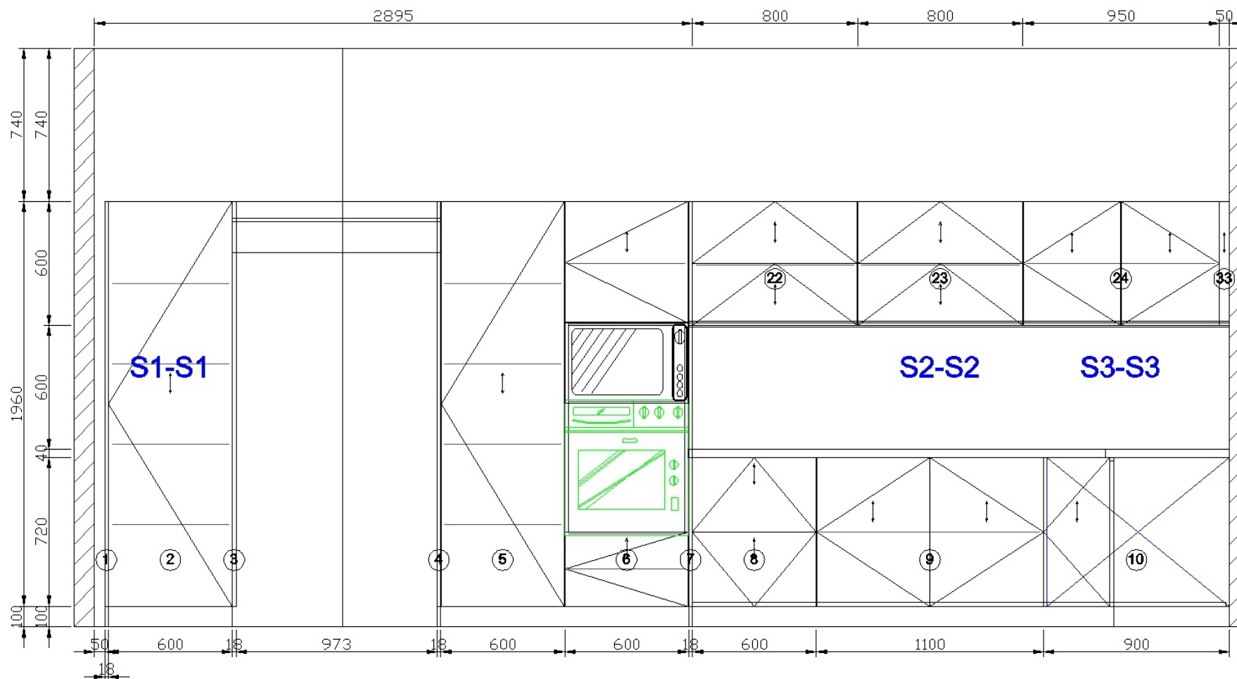
A View elevation drawing
